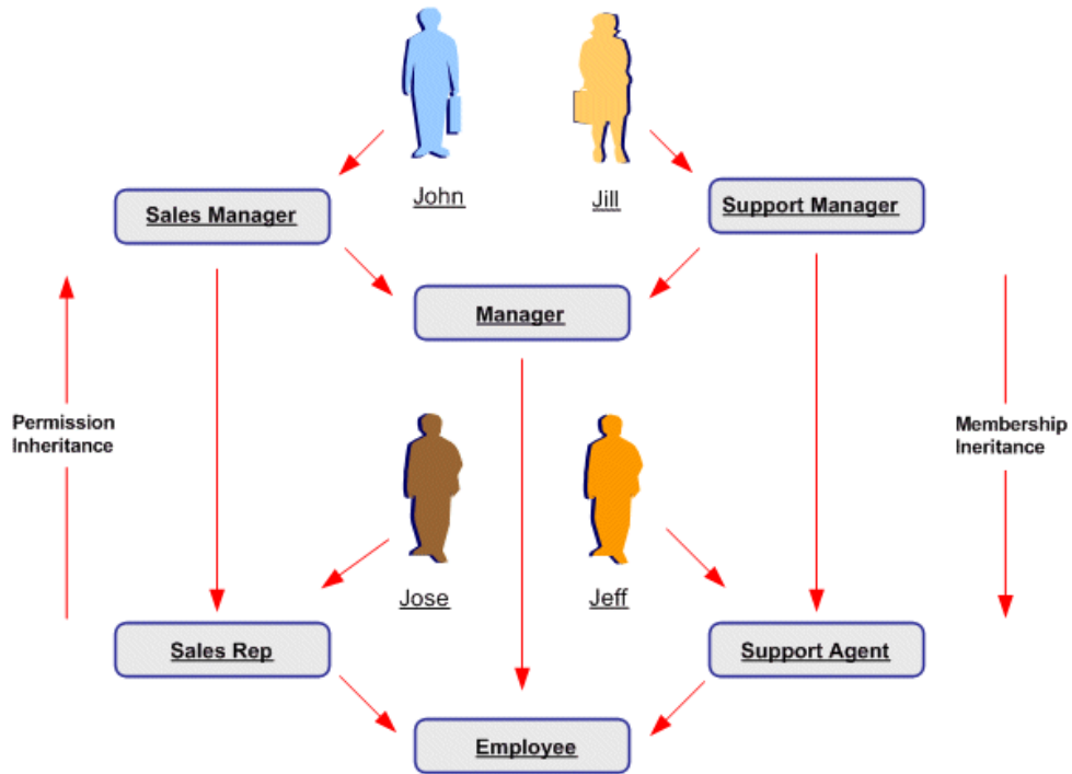
Figure 3-1 Role Inheritance Hierarchies
