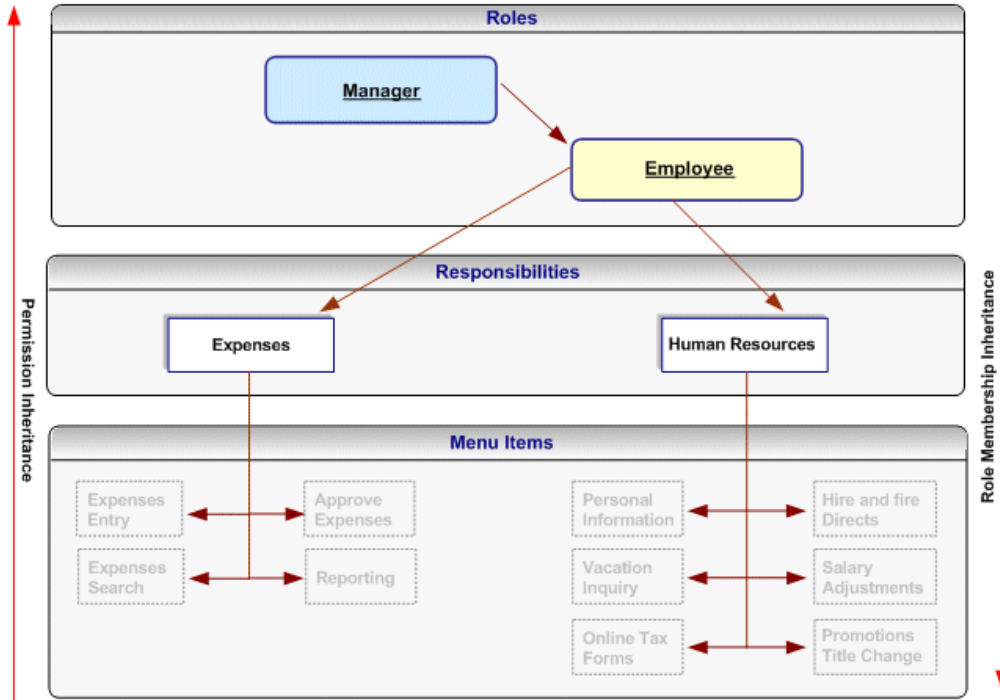
Figure 3-4 Role Inheritance Relationship in Which a Role Inherits the Responsibilities Inherited by its Subordinate Role
